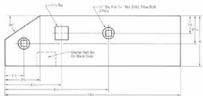
522343 Landside — IHC — "Rear" Landside Right Hand Shown Left Hand Opposite Super Chief Bottom
