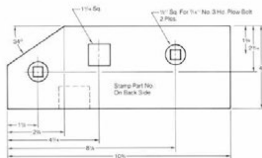
522342 Landside — IHC — "Front" Landside Right Hand Shown Left Hand Opposite Super Chief Bottom
