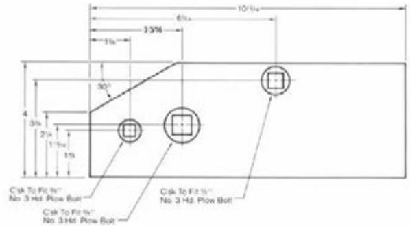
T10856 Landside — CASE PLOWS — Front or Rear Landside for EX Series Bottoms
