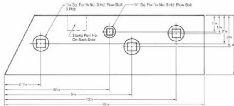
522342 Landside — IHC — "Front" Landside Right Hand Shown Left Hand Opposite Super Chief Bottom
