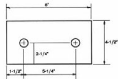
A27862 LANDSIDE 5/8 X 3-1/2-5/8 X 3-1/2
