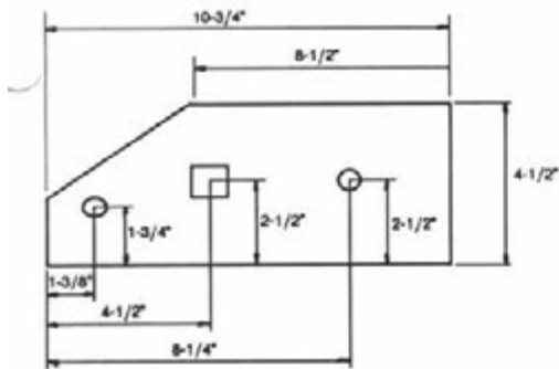
489465 RH LANDSIDE 542417 LH LANDSIDE 7/16 X 1-3/4 - 7/16 X 1-3/4
