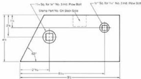
107981 Landside — FORD — Rear Landside After 1958 107981 R.H. Shown 108429 L.H. Opposite General Purpose Bottom
